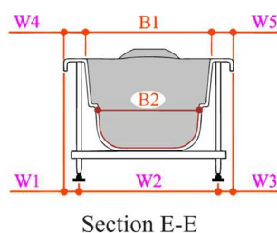
Section E-E
